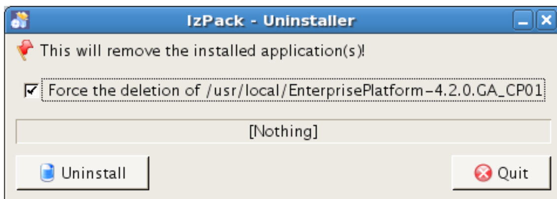
Figure 7.1. Uninstaller
