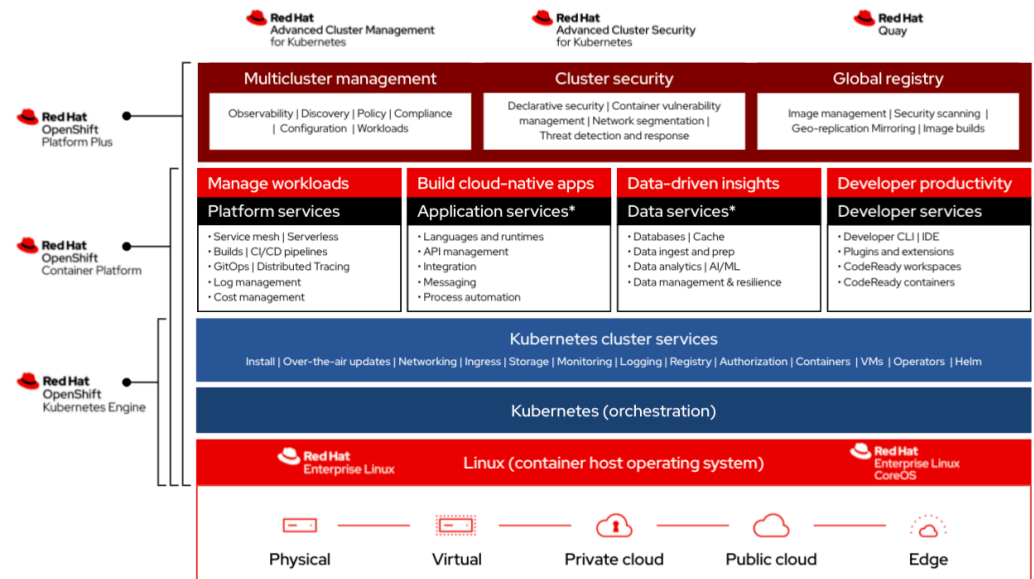
Figure 1. OpenShift Container Platform capabilities and complementary Red Hat products
