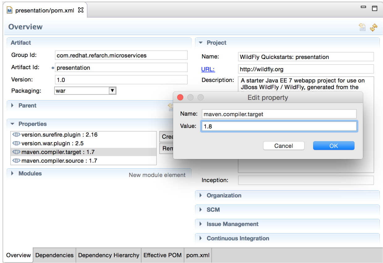
Figure 18. Java version in pom file
